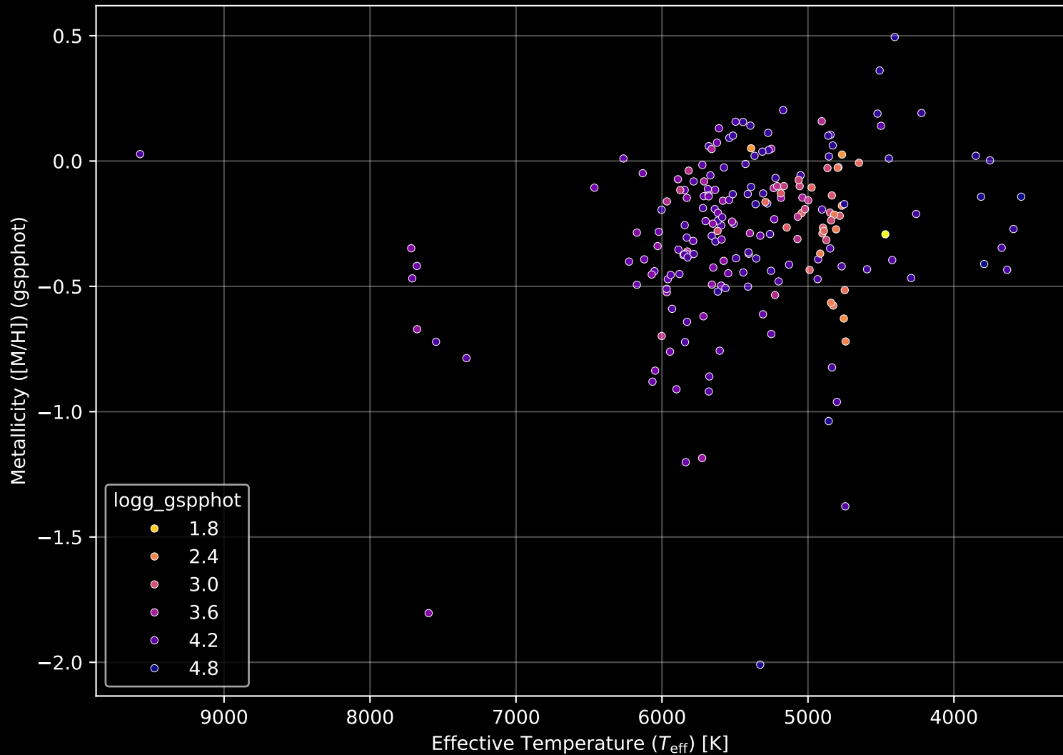
APOGEE DR17 Field: [239+40_MGA] Stellar Population Parameters (n= 203)
