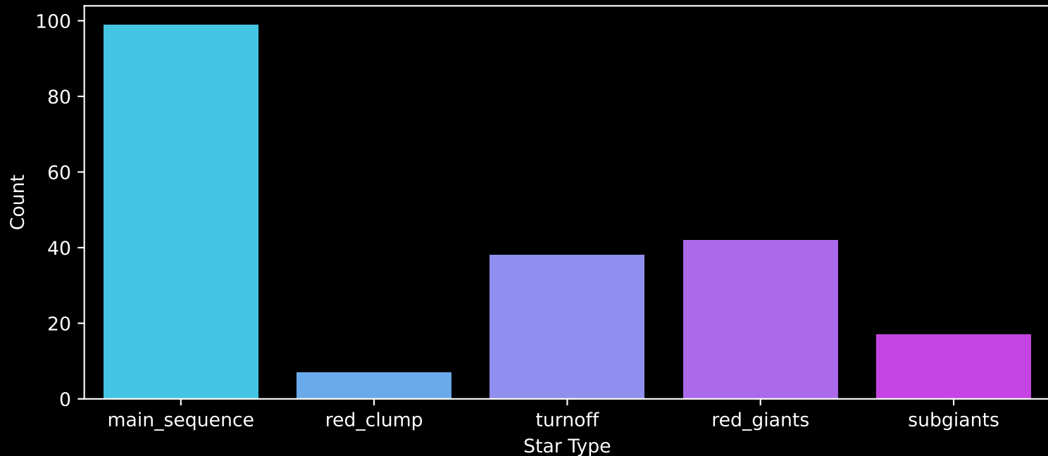
APOGEE DR17 Field: [239+40_MGA] Count plot of Star Type
