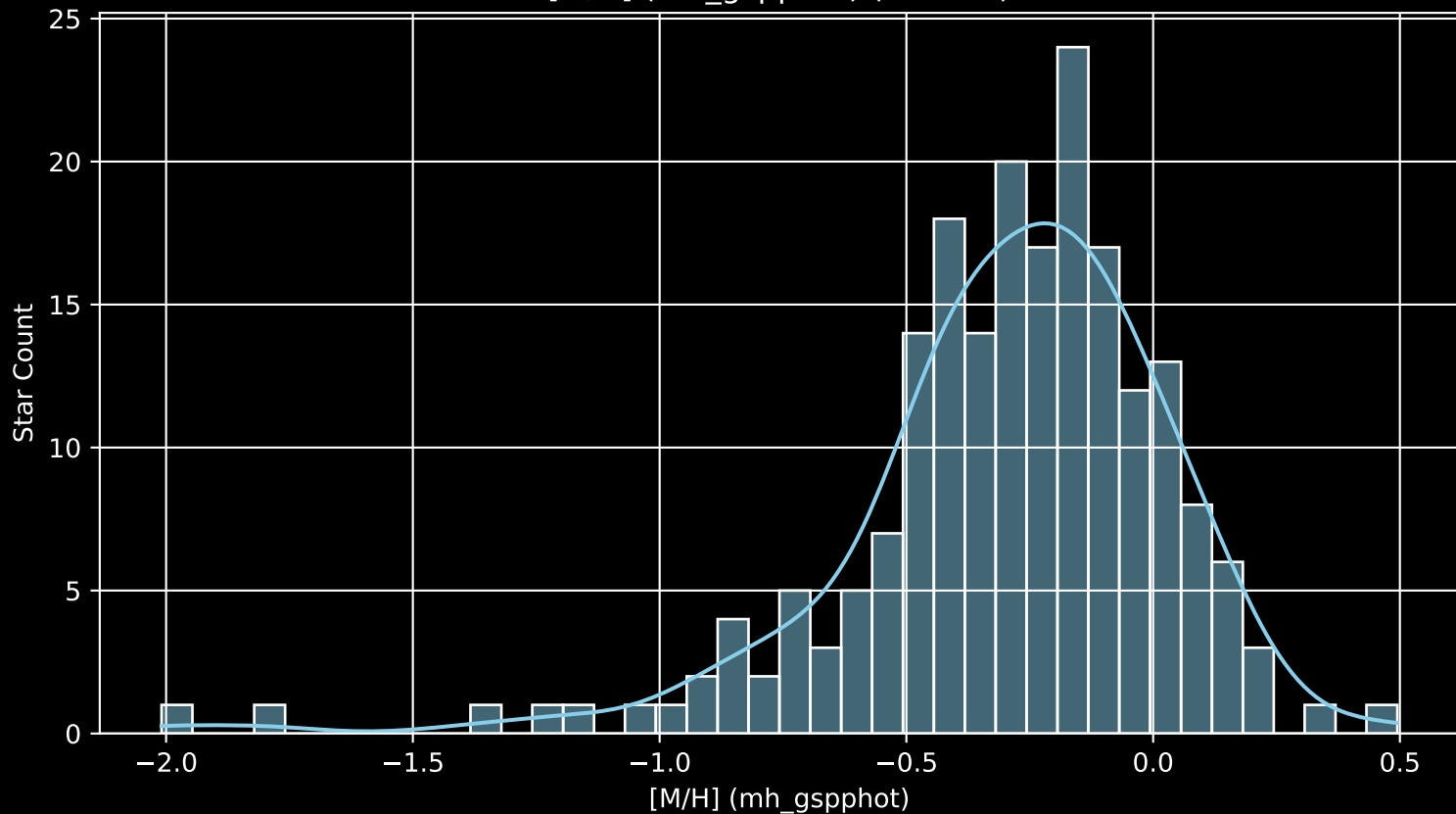
APOGEE DR17 Field: [239+40_MGA [M/H] (mh_gspphot) (n= 203)
