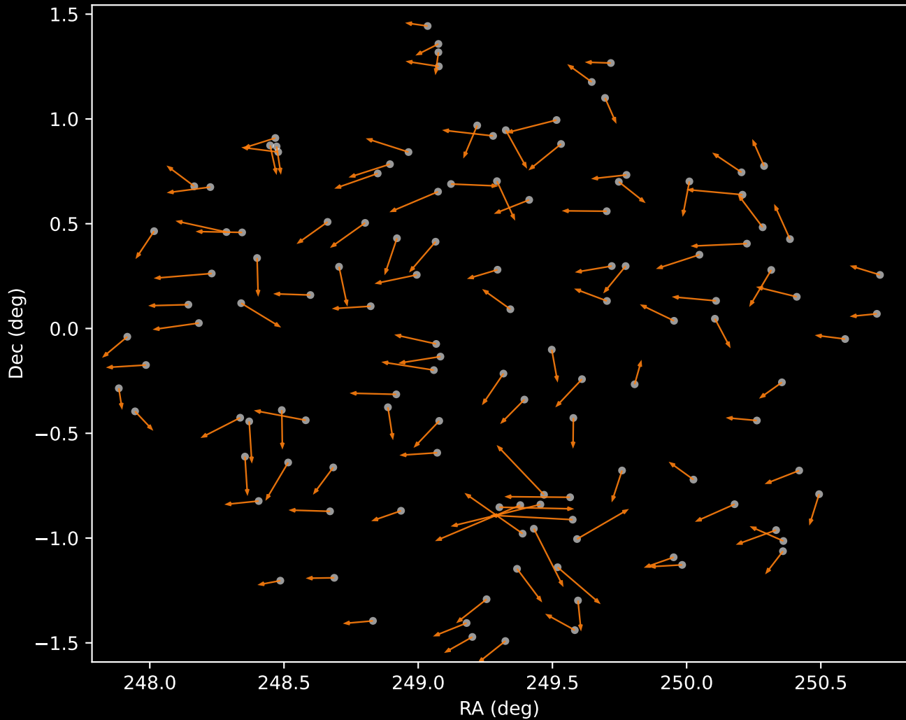
APOGEE DR17 Cluster 2 Proper Motion Vectors (n=124)
