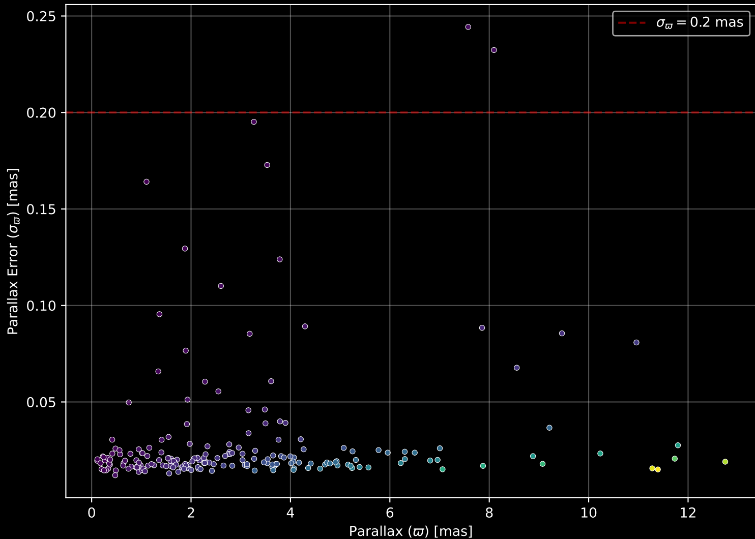
APOGEE DR17 Field: [239+40_MGA] Parallax Quality (n= 203)
