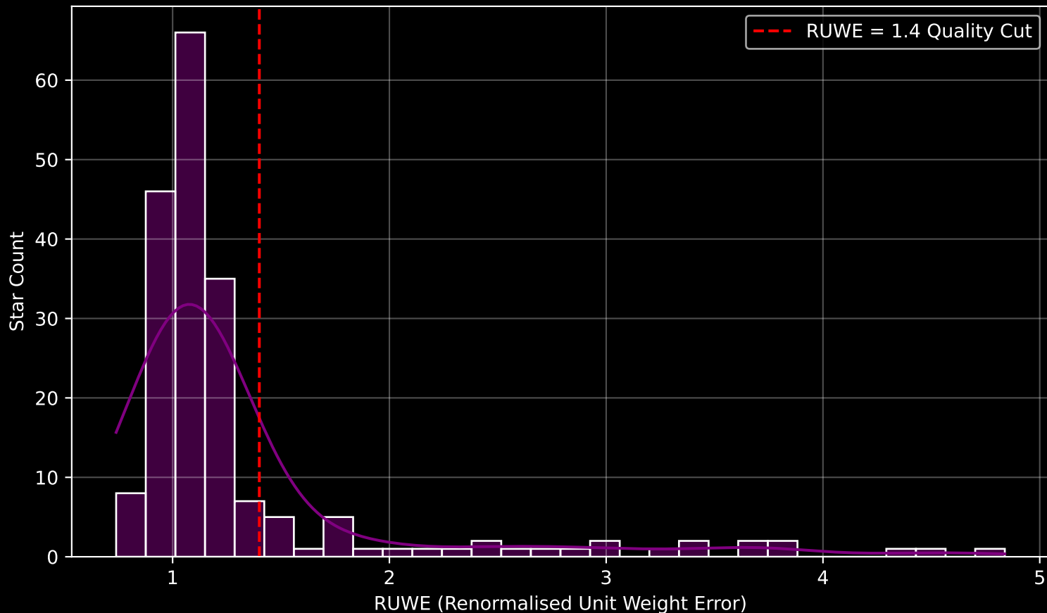
GAPOGEE DR17 Field [239+40_MGA] RUWE Distribution (n= 194)
