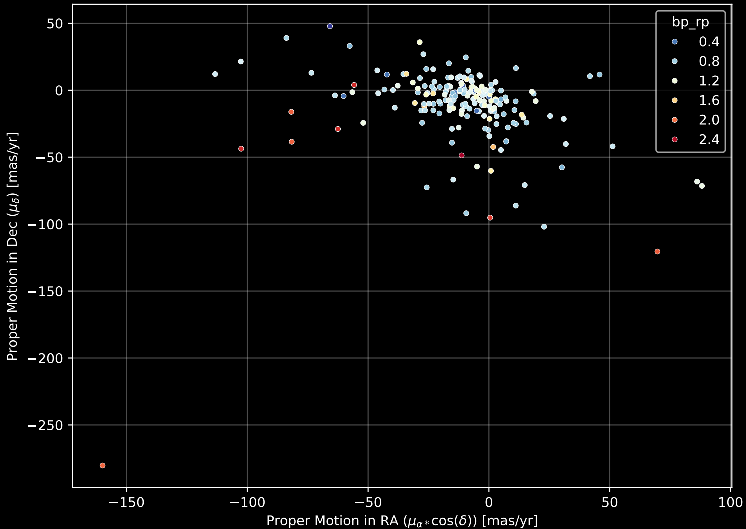
APOGEE DR17 Field: [239+40_MGA] Proper Motion Diagram (n= 203)
